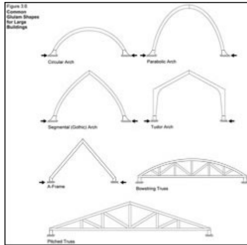
Figure X.X: Common Glulam Shapes for Large Buildings
