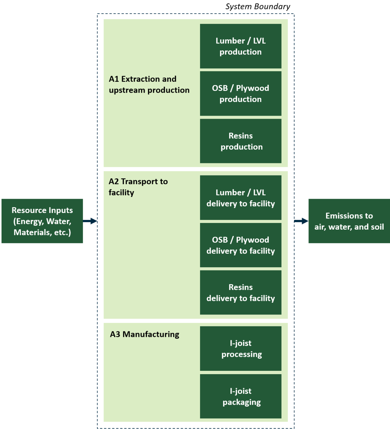
Figure 1. Cradle-to-gate I-joist production flow diagram
